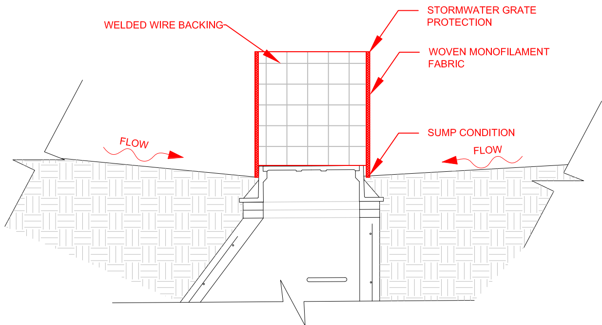
SECTION
