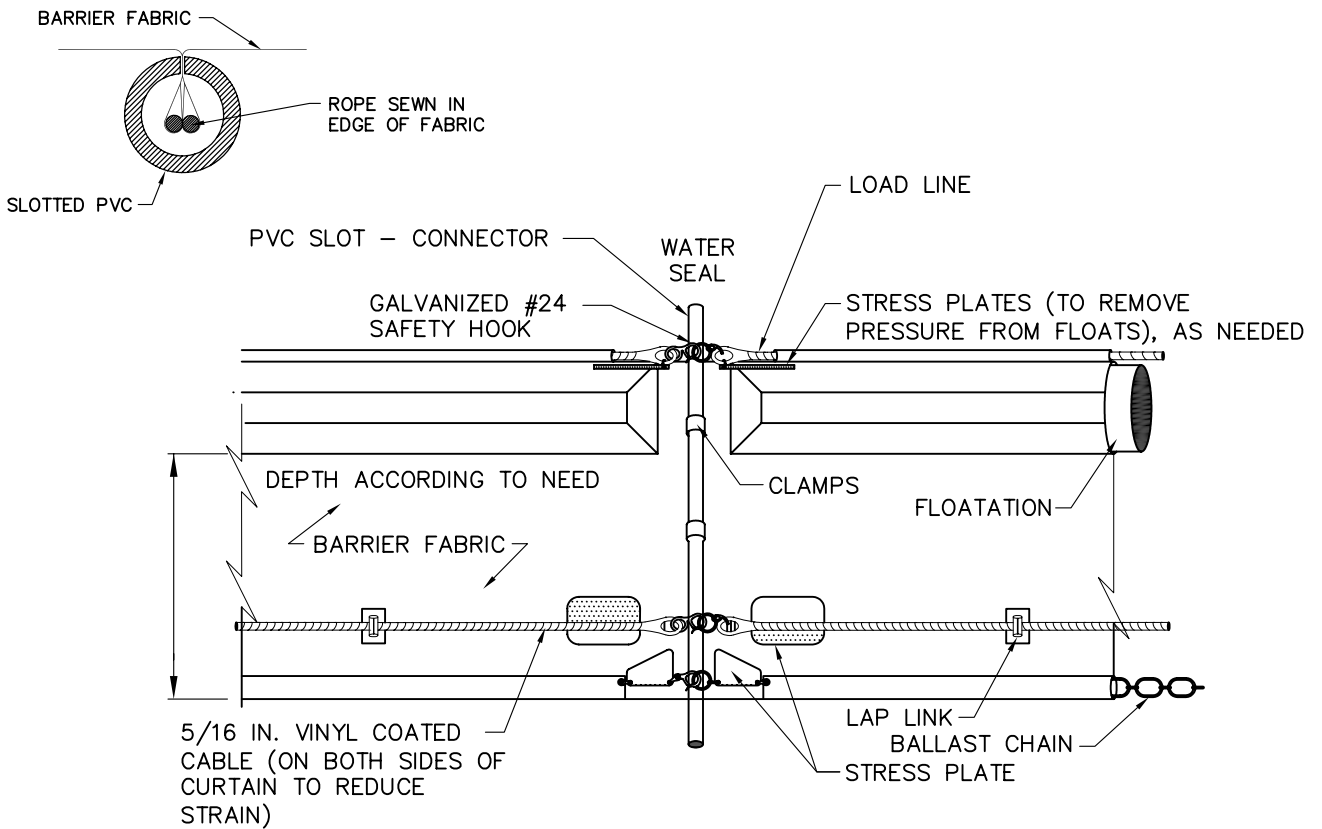
SLOTTED PVC CONNECTOR (SHOWN WITH OPTIONAL REINFORCEMENT)
