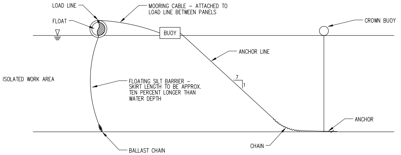
TYPICAL COMPONENTS / ANCHORAGE SYSTEM
