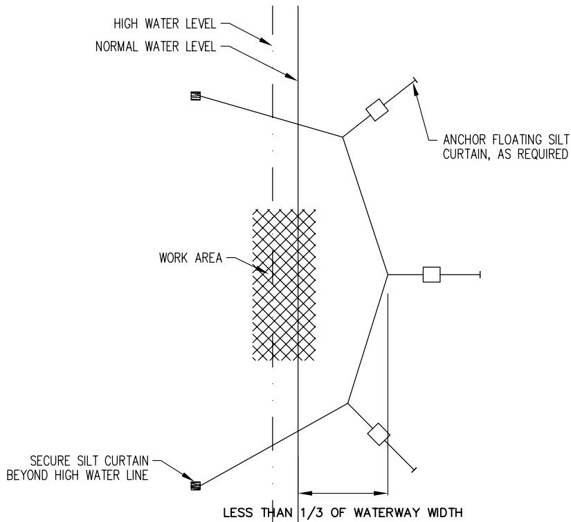
TYPICAL COMPONENTS / ANCHORAGE SYSTEM
