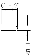
STAPLE DETAIL
